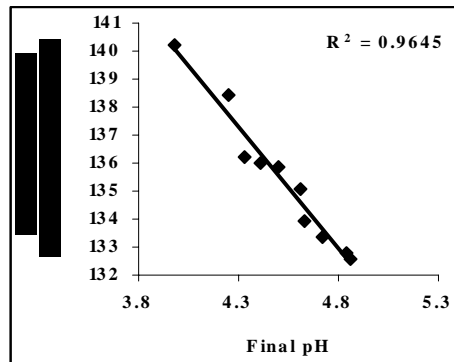
Figure 2: Effect of final solution pH on the concentration of lead dissolved (as obtained from experiment (Nwoye,2008))
