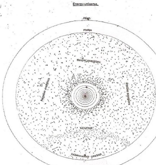
Energy particle has internal structure and having three kinds of basic elements proposed and named as Positive energions (PEONS), Negative energions (NEONS) and Neutral energions (NEUONS). It is also another universe named as Energy-UNIVERSE having structure and properties exactly similar to the structure and properties resembling our Geo-UNIVERSE and Atomic-UNIVERSE.
