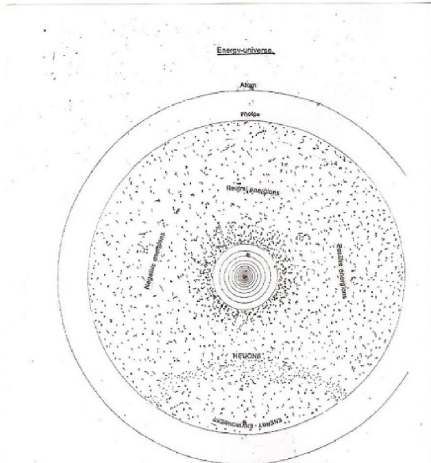
Energy particle has internal structure and having three kinds of basic elements proposed and named as Positive energies (PEONS), Negative energies (NEONS) and Neutral energies (NEUCONS); it is also another universe named as Energy-UNIVERSE having structure and properties exactly similar to the structure and properties resembling our Geo-UNIVERSE and Atomic-UNIVERSE.
