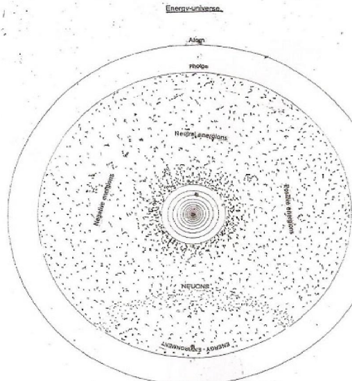
Energy particle has atomic structure and having three kinds of basic elements proposed and named as Positive energions (PEONS), Negative energions (NEONS) and Neutral energions (NEUCONS). It is also another universe named as Energy-UNIVERSE having structure and properties exactly similar to the structure and properties resembling our Geo-UNIVERSE and Atomic-UNIVERSE.
