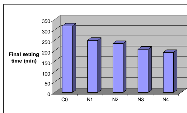
Figure 2. Influence of nano-Al 2 O 3 particles on the final setting time of cement paste.
