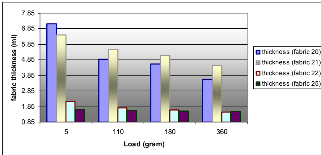
Figure 4: Loads Vs Thickness of fabrics
