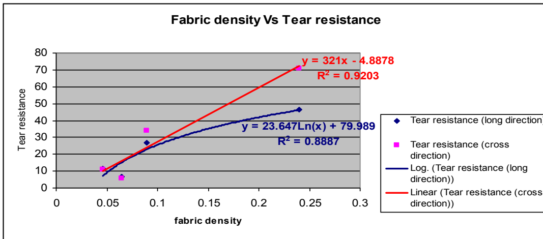
Figure 10: fabric density Vs fabric tear resistance
