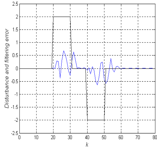
Figure 4 Disturbance and filtering error (Constant delay case)
