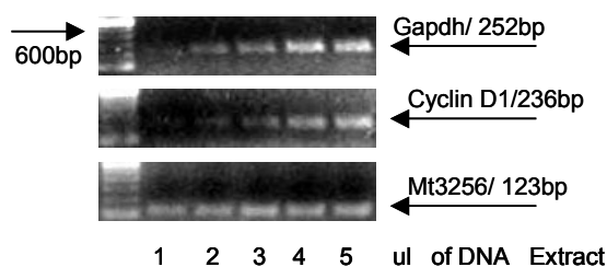
Figure 3A. Primer expression on DNA volume-dependent effective with the DNA extract from human blood
