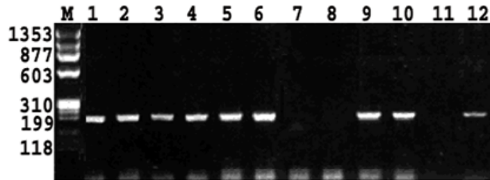
Figure 1. Detection of TTV-DNA by nested PCR. PCR products were separated on 1.5% agarose gel electrophoresis and were stained with ethidium bromide . Lanes 1,2,4,3,4,5,6,9,12, show positive TTV DNA viraemia at 199 bp. Lane 7,8 Negative TTV-DNA. Lane 10,11 positive and negative control respectively.
