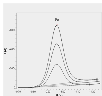
Figure 2. Voltammogram of Fe in Tap water.
