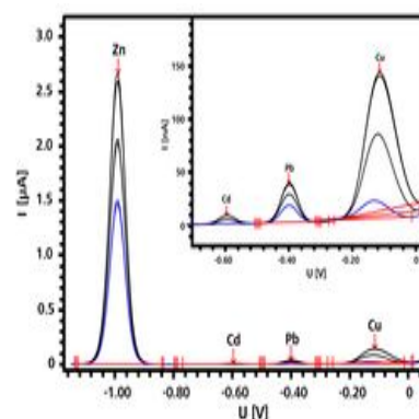
Figure 1. Voltammogram of the trace elements (Cu, Pb, Cd, Zn) in Tap water.
