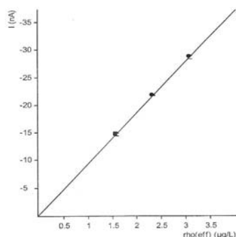
Figure 5. Plot of concentration (µ/l) and current (nA) Se element in Tap water.
