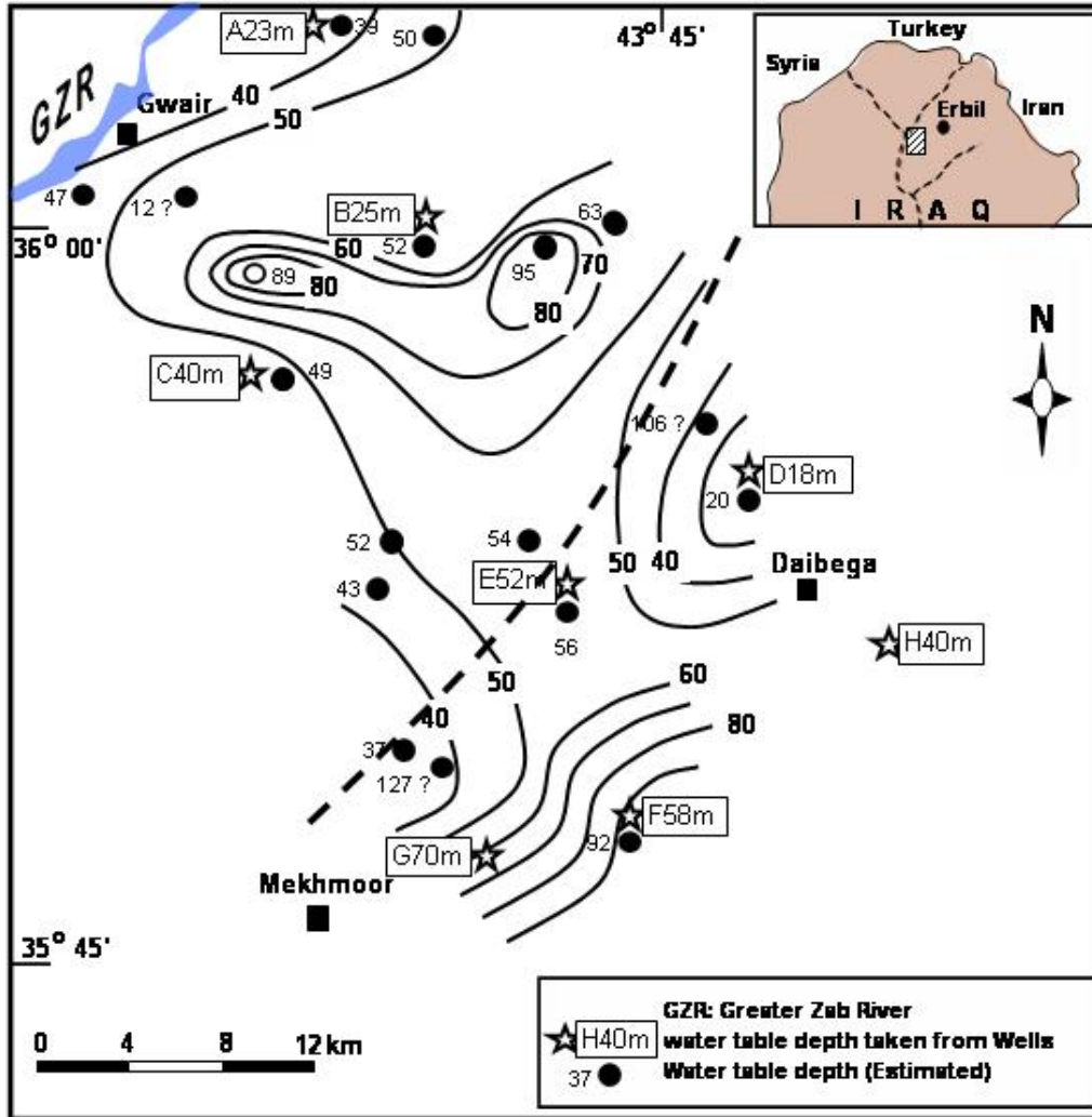
Fig. 8: Water Table Depth Map Estimated from Resistivity Data
