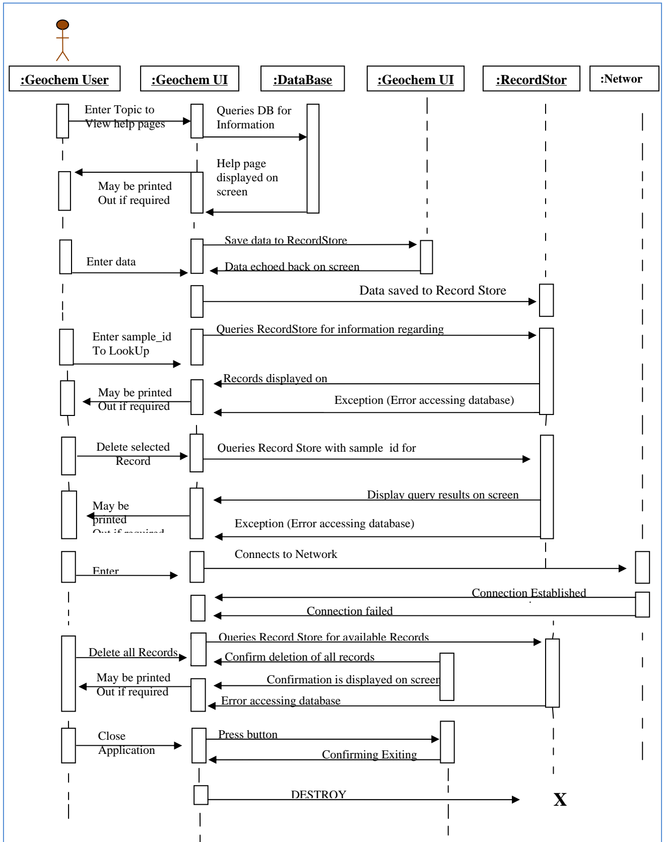
Figure 6. A typical Sequence Diagram with objects and messages
