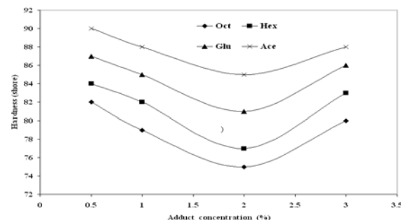
Figure (2): The effect of different types of adducts on the hardness of the treated leather.
