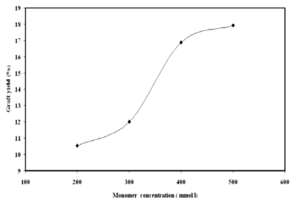
Figure (7): The effect of VP concentration on the GY % of grafted leather.
