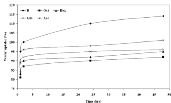
Figure (3): The effect of different types of adducts on the water uptake % of the treated leather.
