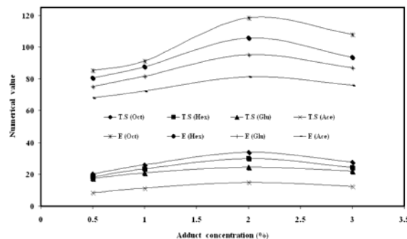
Figure (1): The effect of different type of adducts on the tensile strength and elongation % of treated leather.
