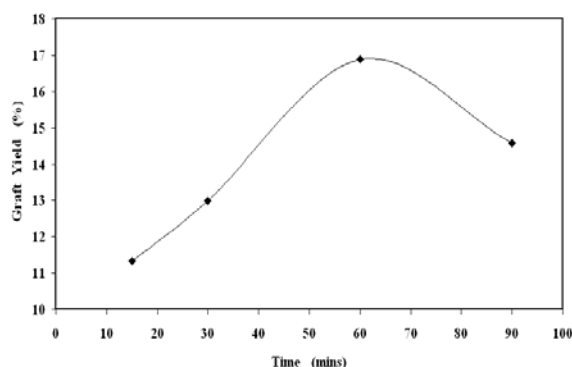
Figure (5): The effect of reaction time on the GY % of grafted leather.
