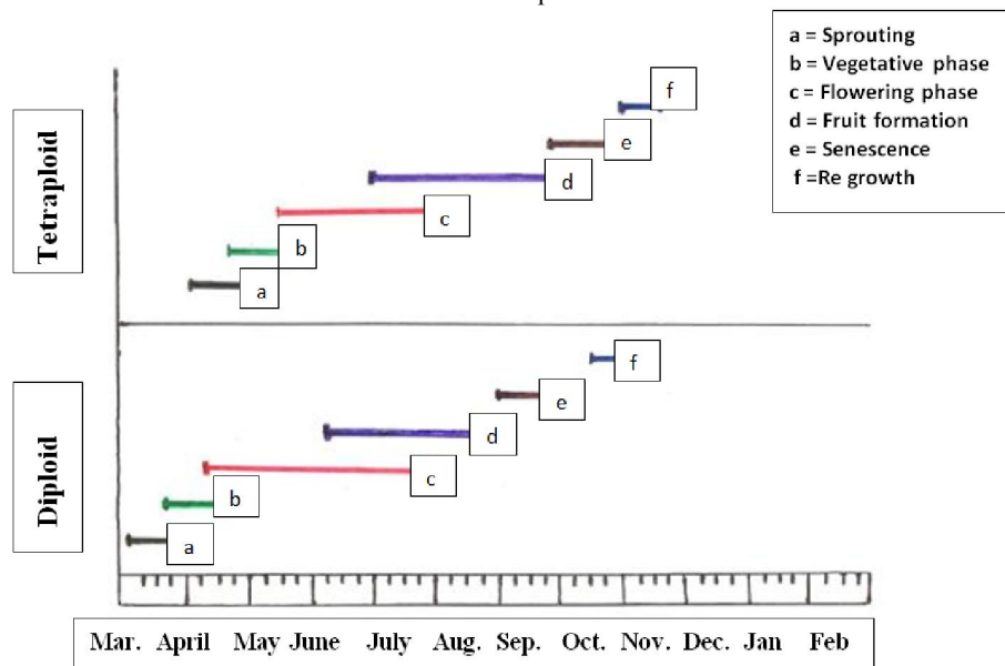
Fig. 1: Phenogram of Diploid and tetraploids population of Peganum harmala
