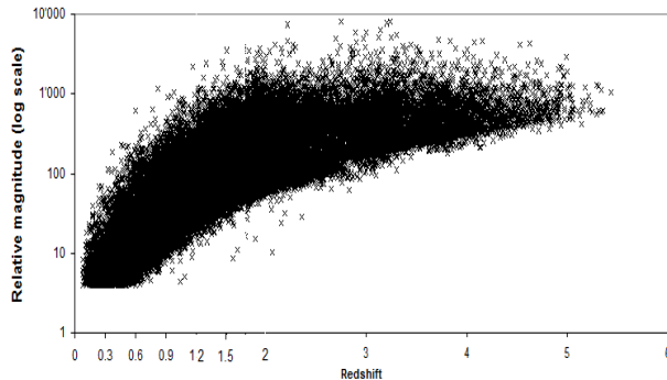
Figure 4: Plot of individual quasar relative magnitude versus redshift.
