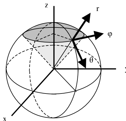
Figure 1: Representation of a conical observation in spherical coordinates, where r is the radius, \phi is azimuth between [0, 2\pi] , and \theta the zenith angle is between [0, \theta_0] with \theta_0 the interior angle of the cone.
