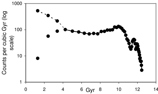
Figure 3: Density-distance curve derived from the equivalent spherical sampling, where Gyr are billion light years from today. Distances are computed from redshift conversion with the calculator of Wright (2006). Bright quasar observations below 4 Gyr appear to be biased due to the cut-off for small relative magnitude quasars (figure 4). The dotted line includes faint magnitude quasars retrieved from the CAS.
