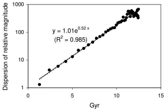
Figure 6: Dispersion of quasar relative magnitude (log-scale) versus light travel distance in Gyr. The dispersion was measured as the sample standard deviation for buckets of redshift width 0.1. Note that for the regression, the part of the curve with redshift above 4.7 was excluded due to noise and non linearity.
