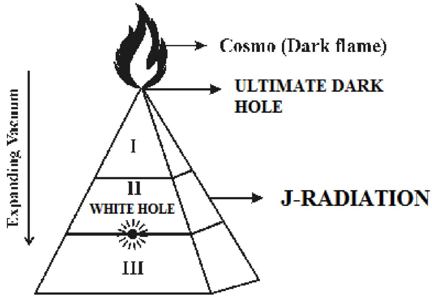
(MODEL COSMO UNIVERSE)
