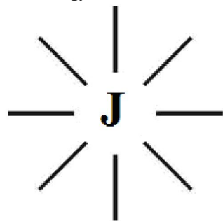
GOD OF UNIVERSE (Joule)
