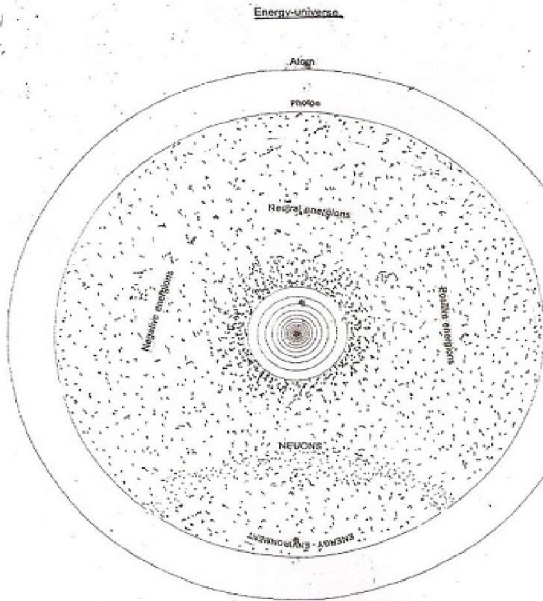
Energy particle has internal structure and having three kinds of basic elements proposed and named as Positive energies (PEONS), Negative-energies (NEONS) and Neutral-energies (NEUONS). It is also another universe named as Energy-UNIVERSE having structure and properties exactly similar to the structure and properties resembling our Geo-UNIVERSE and Atomic-UNIVERSE.
