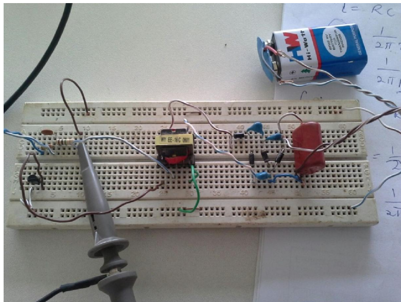
Figure 4. Assembly of temporary circuit
