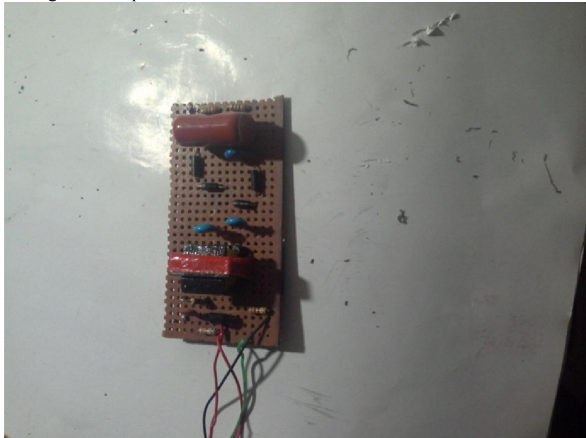
Figure 6. Zapper circuit on permanent (vero) board
