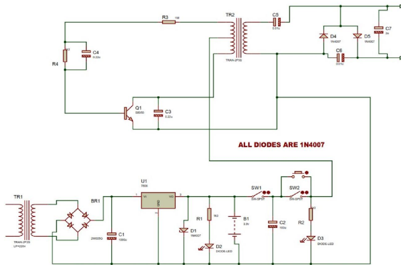
Figure 1. General Zapper circuit diagram
