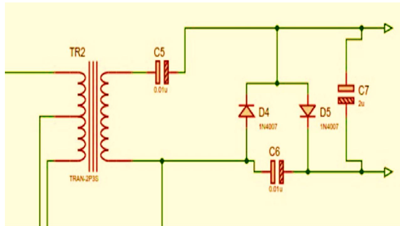
Figure 2. Transformer and Tripler Circuit Diagram
