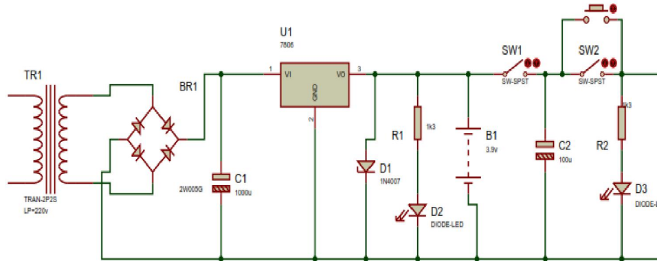
Figure 3. Power supply unit
