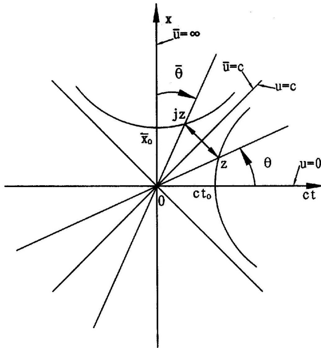
Fig. 1. Mathematical theory of space-time
