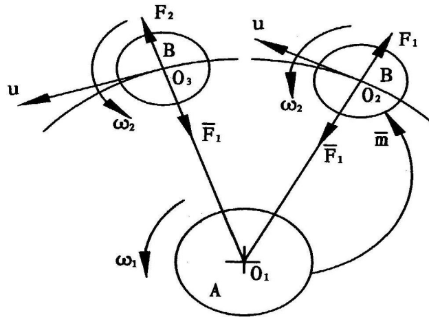
Fig. 4. A expansion model of the Universe
