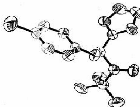
Fig 3 ORTEP diagram of tridimefon
