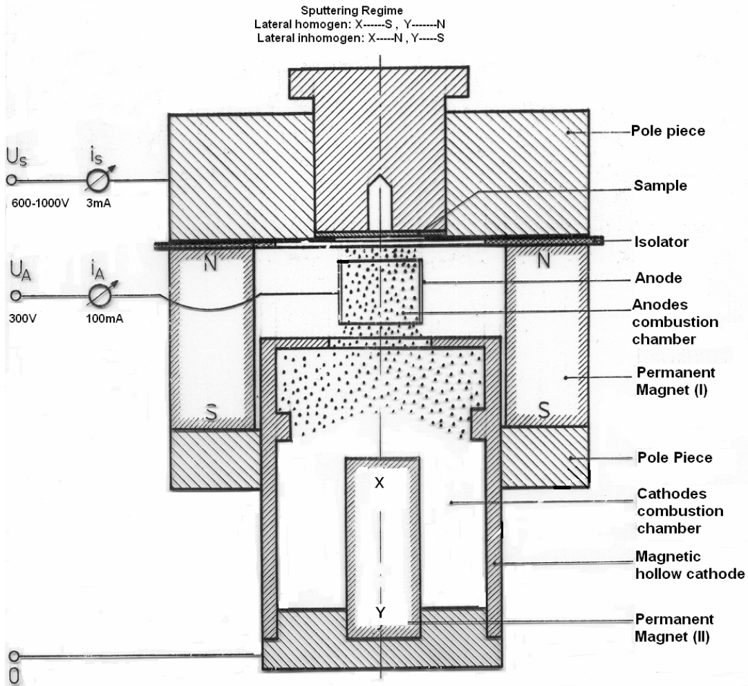
Figure 1: Sputtering arrangement with magnetic hollow cathode
