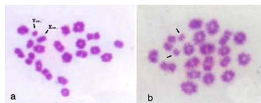
Figure 3: Metaphases spread from mice spermatocytes showing (a) XY univalents, (b) Autosomal univalents after treatment with 1\text{mg TMT/ kg b.wt.}
