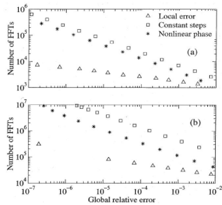
Fig. 1. Plot of the total number of FFTs versus global relative error \varepsilon for (a) second-order and (b) fifth-order solitons.
