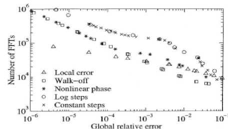
Fig. 5. Plot of the total number of FFTs versus global relative error " for the multichannel CRZ system.
