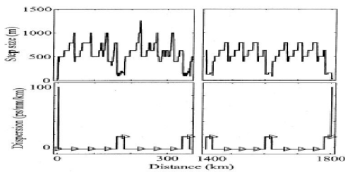
Fig. 6. Step size h as a function of distance for the local-error method applied to the multichannel CRZ system.
