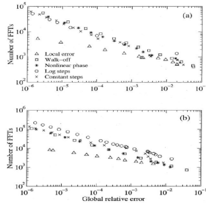
Fig. 4. Plot of the total number of FFTs versus global relative error " for the single-channel (a) DMS and (b) CRZ systems.
