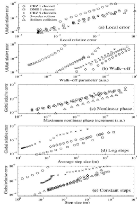
Fig. 7. Plot of the global error as a function of method parameter for (a) local error, (b) walk-off, (c) nonlinear phase, (d) logarithmic step, and (e) constant step methods.
