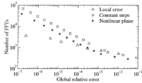
size method. Fig. 2. Plot of the total number of FFTs versus global relative error for a collision of two first-order solitons.
