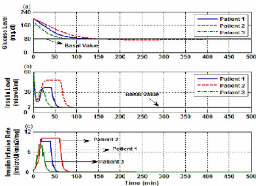
Fig. 5 Closed-loop glucose regulatory system.(a) Plasma glucose concentration. (b) Plasma insulin concentration (c) Exogenous insulin infusion rate.
