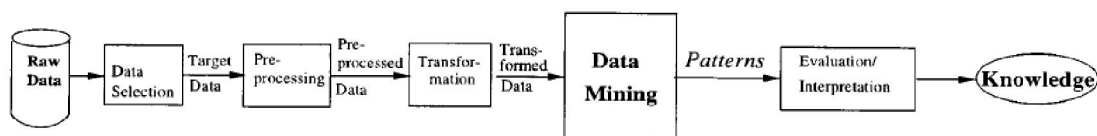
Figure 1: KDD process
