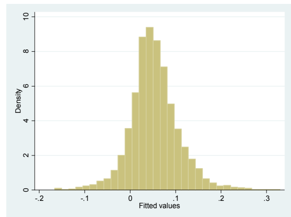
Figure (1) the normal histogram of remained in Dichow and Dichow models
