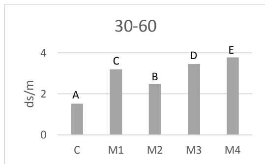
Graph 12- SAR in depth of 30-60cm
