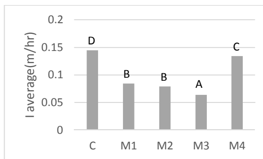
Graph 2- average infiltration rate in mid-season
