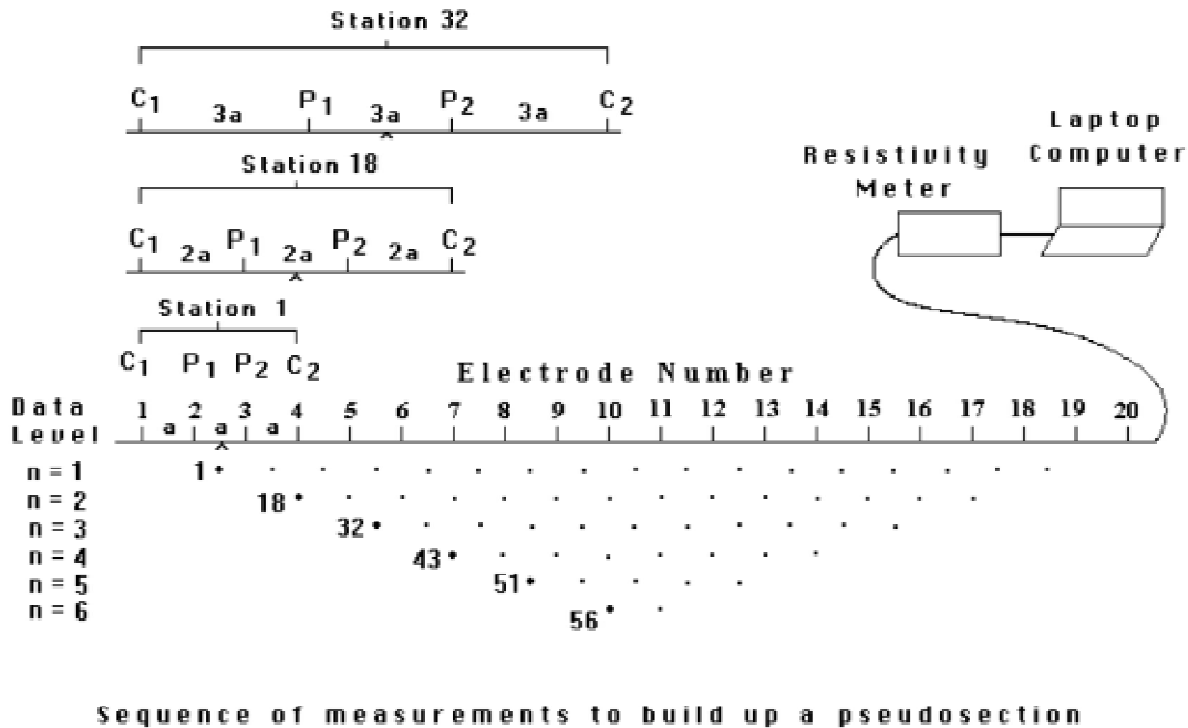
Figure 1.2 Sequence of measurement to build up a pseudosection
