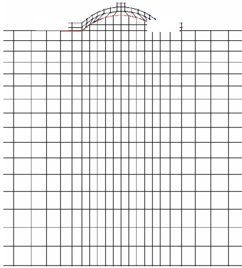
(1-a) Proposed finite-infinite element mesh
