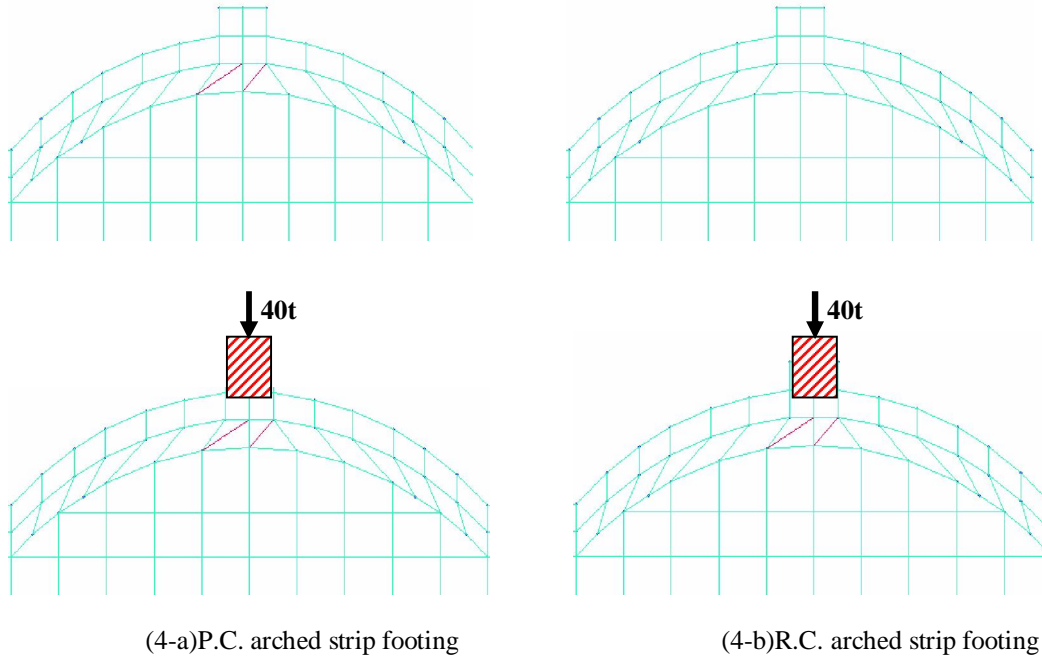
Fig. 4. Crack pattern for P.C. & R.C. arched strip footing for different loads at ratio (t/B) = 0.1 , (h/B) = 0.2 and silty clay soil.
