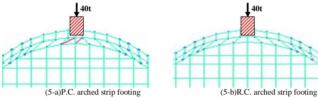
Fig. 5. Crack pattern for P.C. & R.C. arched strip footing for different loads at ratio (t/B) = 0.1 , (h/B) = 0.2 and silty sand soil.
