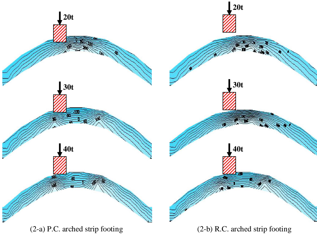
Fig. 2. Effect of load increasing on the normal stress ( \sigma_x ) contour in R.C. & P.C arched strip footing at ratio (t/B) = 0.1 , (h/B) = 0.2 and silty clay soil.
