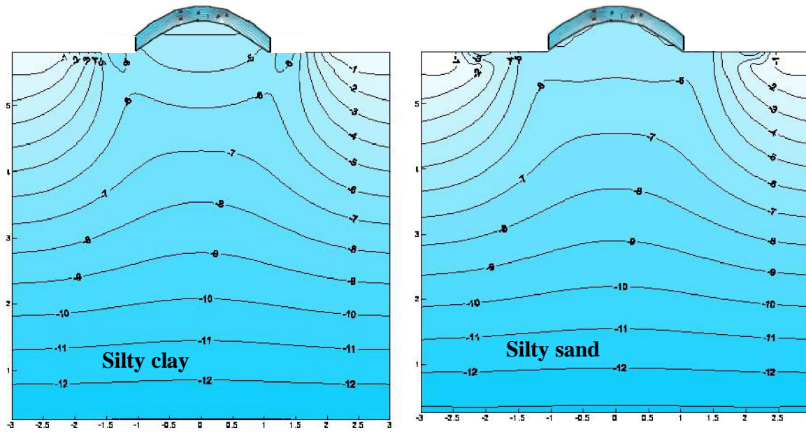
(6-a) P.C. arched strip footing
