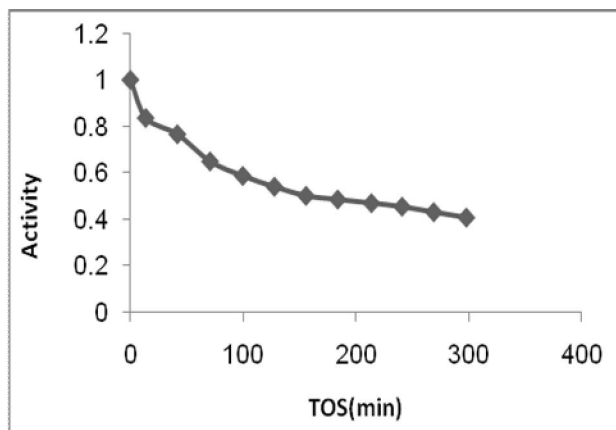
Fig 4. Deactivation rate of FeMo catalyst
