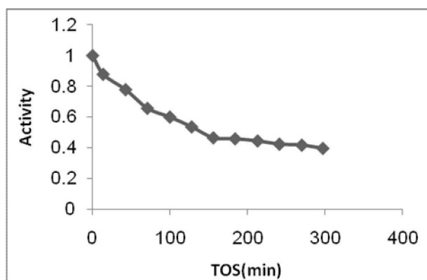
Fig 5. Deactivation rate of FeTa catalyst
