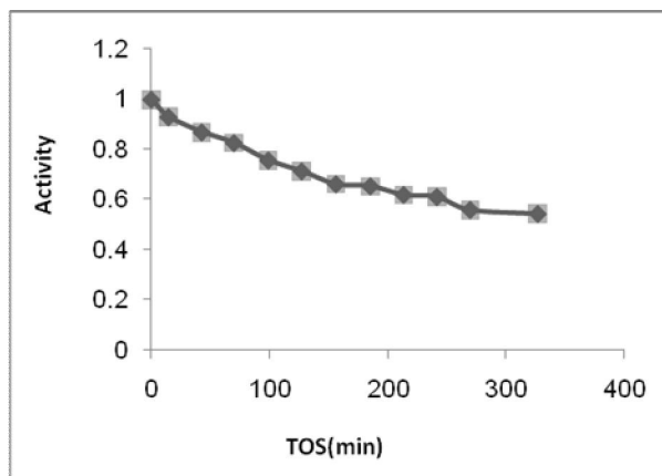
Fig 1. Deactivation rate of Fe 100 catalyst
