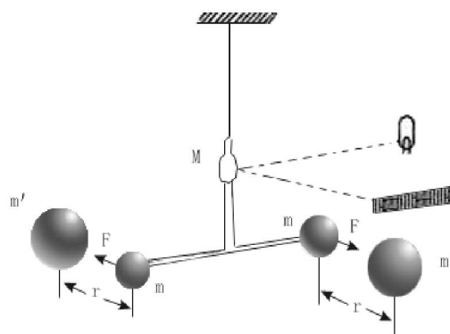
Schematic diagram of Cavendish
