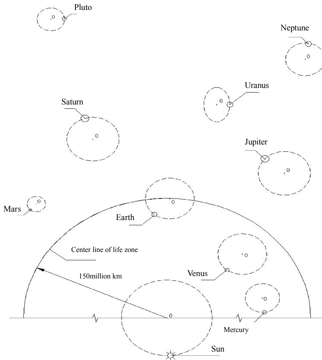
Fig.1 Celestial movement of half a solar system
