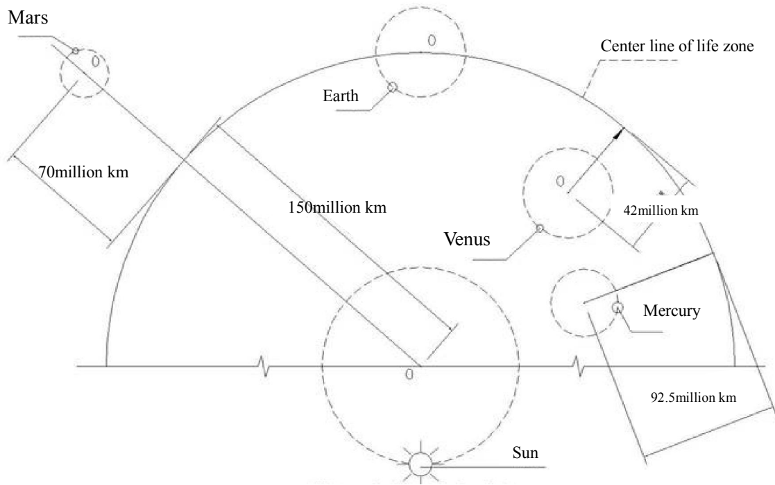
Fig.2 Schematic drawing of moving terrestrial planet
