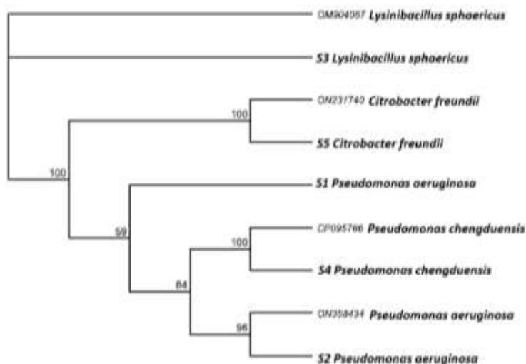
Fig 3.2. Phylogenetic Tree showing evolutionary relationship between isolates
