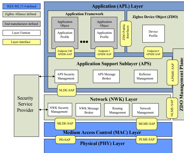
Figure 4. ZigBee stack.
