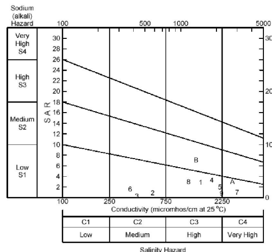
Figure 3. Classification of irrigation waters using U.S. Salinity diagram.
