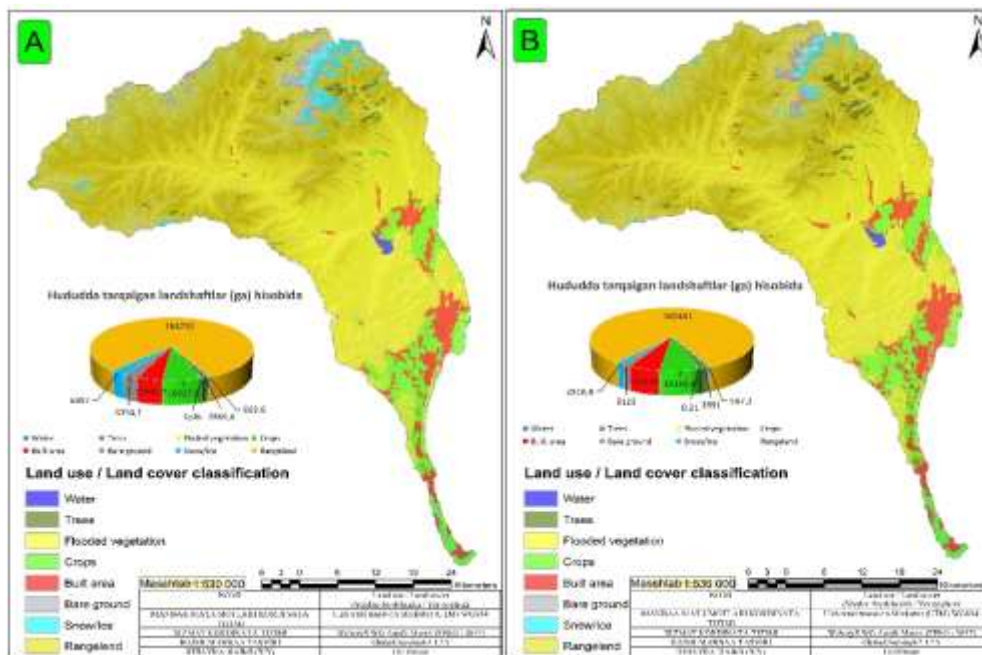
Figure 3. Land Use/Land Cover (LULC) map of the Kosonsoy River Basin (A = 2017; B = 2024)
