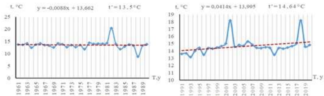
a) Fedchenko meteorological station
