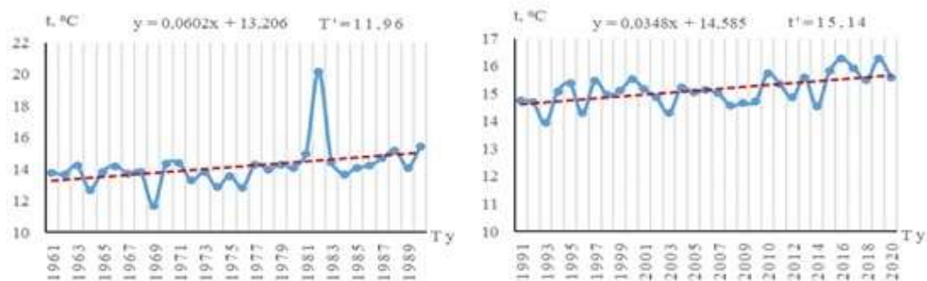
e) Kokand meteorological station
