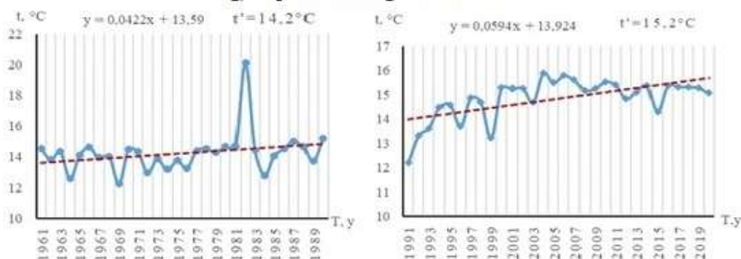
h) Namangan meteorological station
