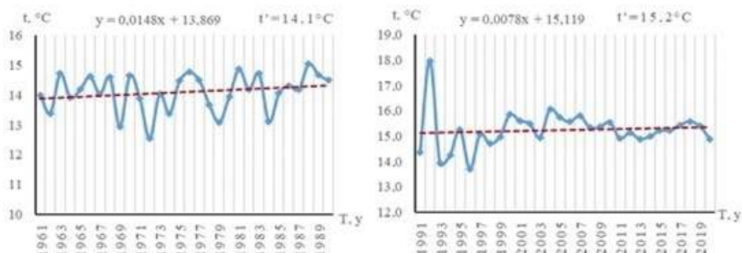
g) Pap meteorological station
