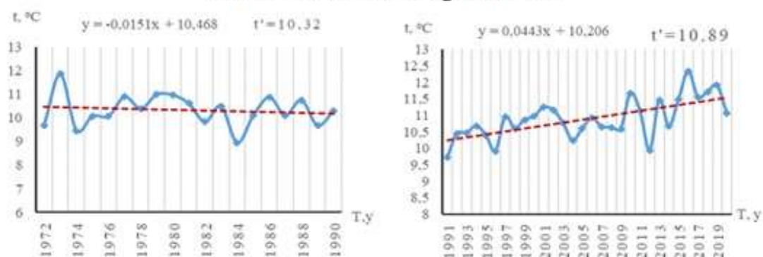
b) Sokh meteorological station
