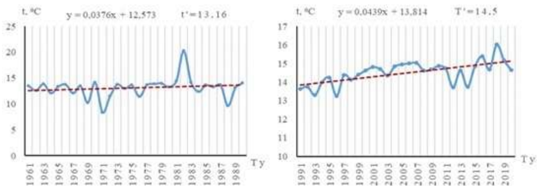
d) Andijan meteorological station
