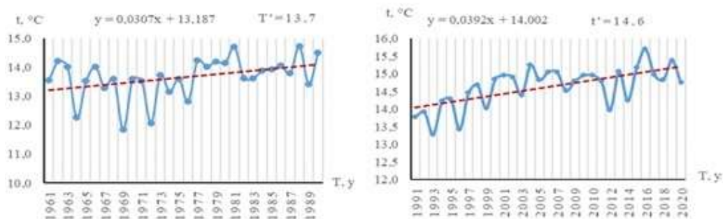
f) Fergana meteorological station
