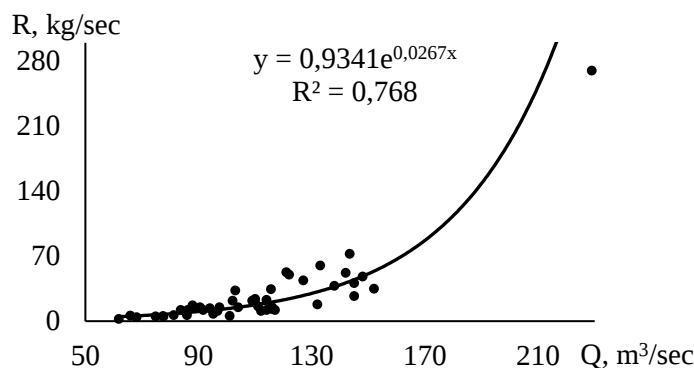
Fig.4. Relationship between suspended sediment runoff (R) and water flow (Q), Chotqol-Khudaydadsay
