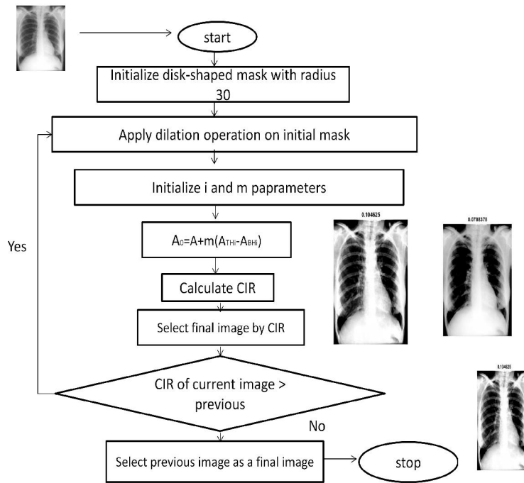
Fig. 6 Enhancement Technique
