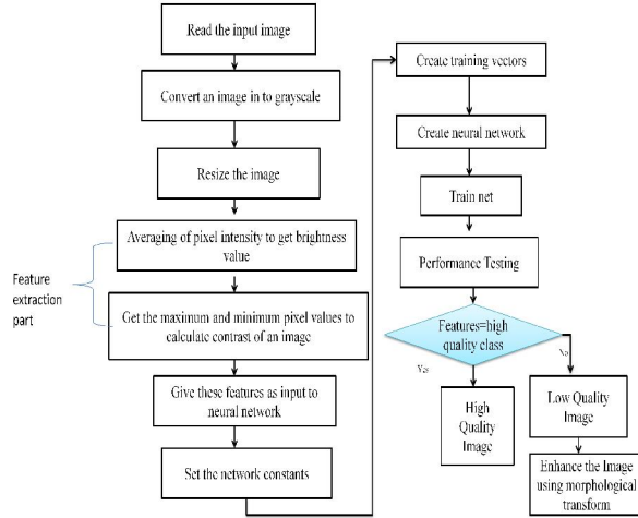
Fig. 4 Proposed work
