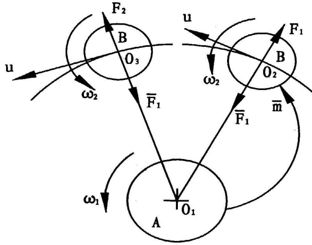
Fig. 4. A expansion model of the Universe
