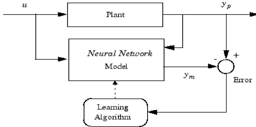
Figure 3. Block diagram of the predictive controller
