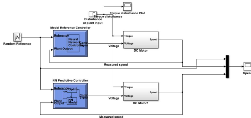
Figure 4 DC motor with Model Reference and Predictive controllers using random reference input
