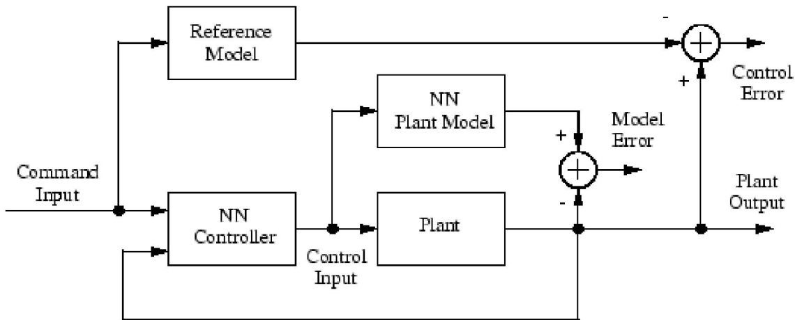
Figure 2. Block diagram of the model reference controller
