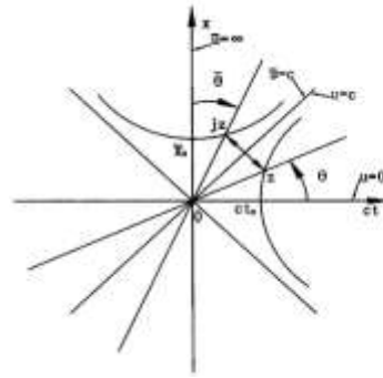
Fig. 1. The Mathematical theory of the space-time with SASC
