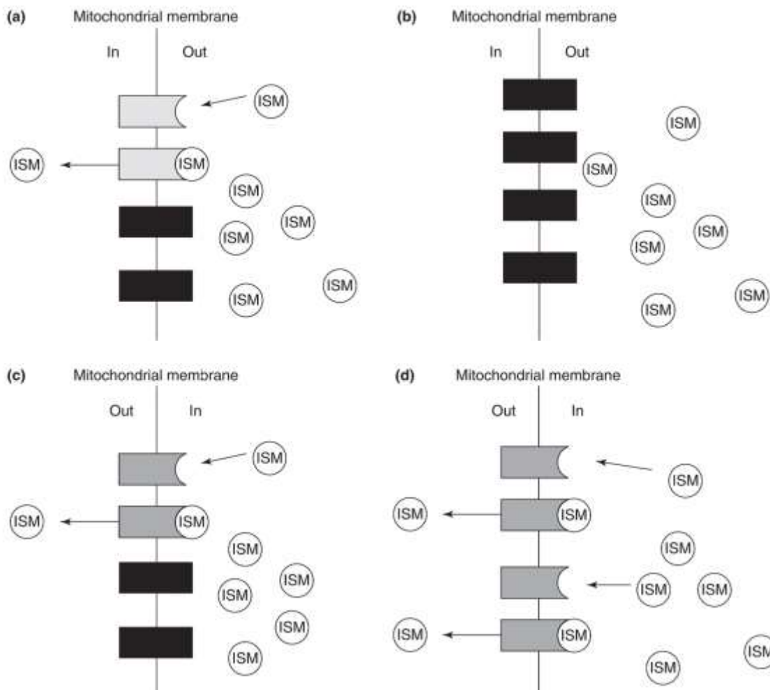
Figure 4: Model of the uptake of ISM by T. congolense mitochondria (Delespaux et al. , 2008).
