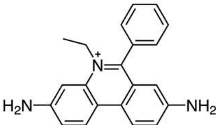
Figure 3. Molecular structure of homidium (Delespau et al. , 2010)
