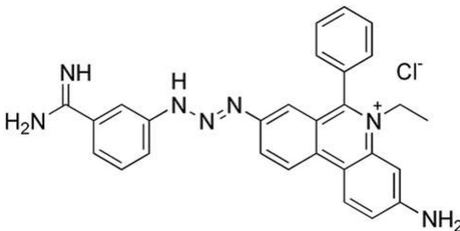
Figure 2. Molecular structure of Isometamidium chloride (Delespau et al. , 2010)
