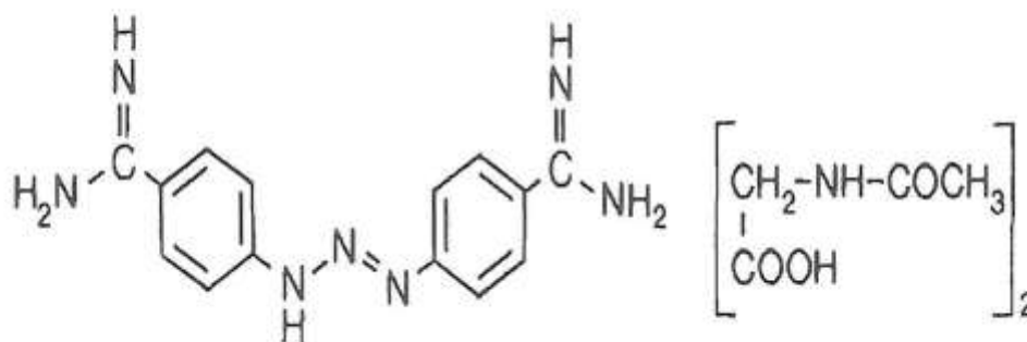
Figure 1. Molecular structure of Diaminazene acetate (Peregrine and Mamman, 1993).
