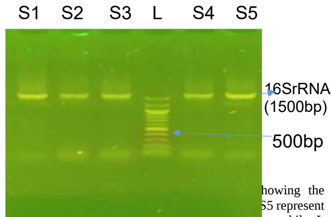
Fig 3.3: Decolourization of Disperse Red by Bacterial Consortium under Anaerobic Condition
